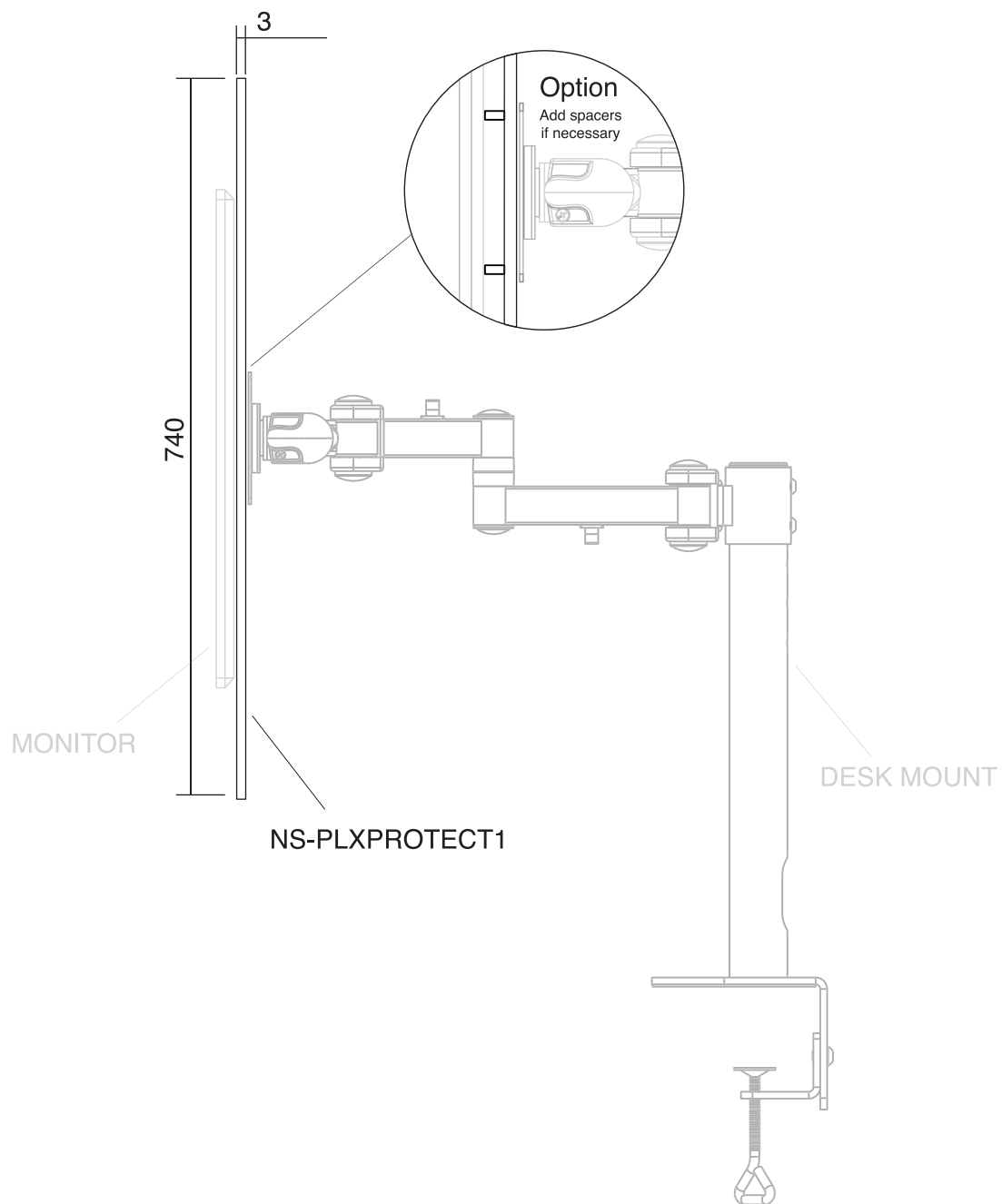
Side view
